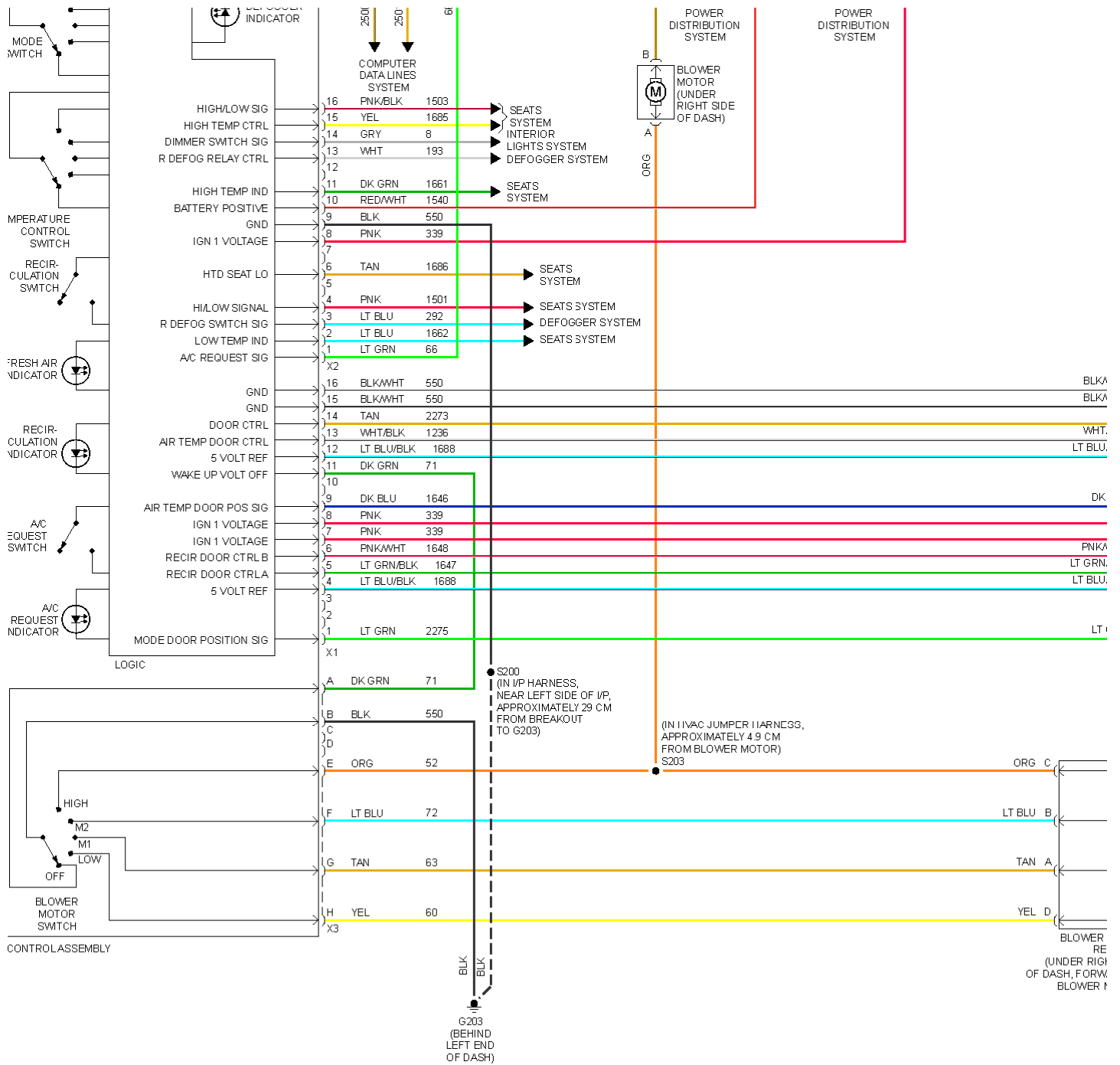
Fig. 2: Manual A/C Circuit (1 of 2)
