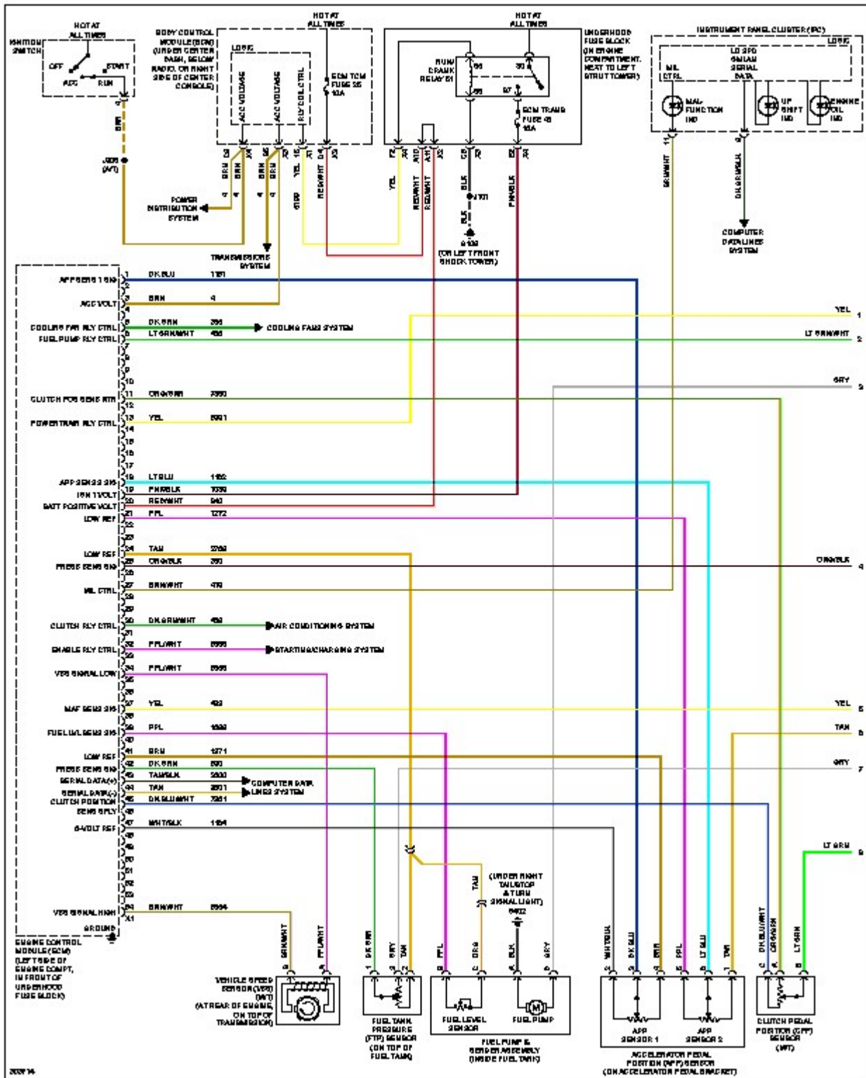
Fig. 25: 2.4L VIN V, Engine Performance Circuit (1 of 4)
