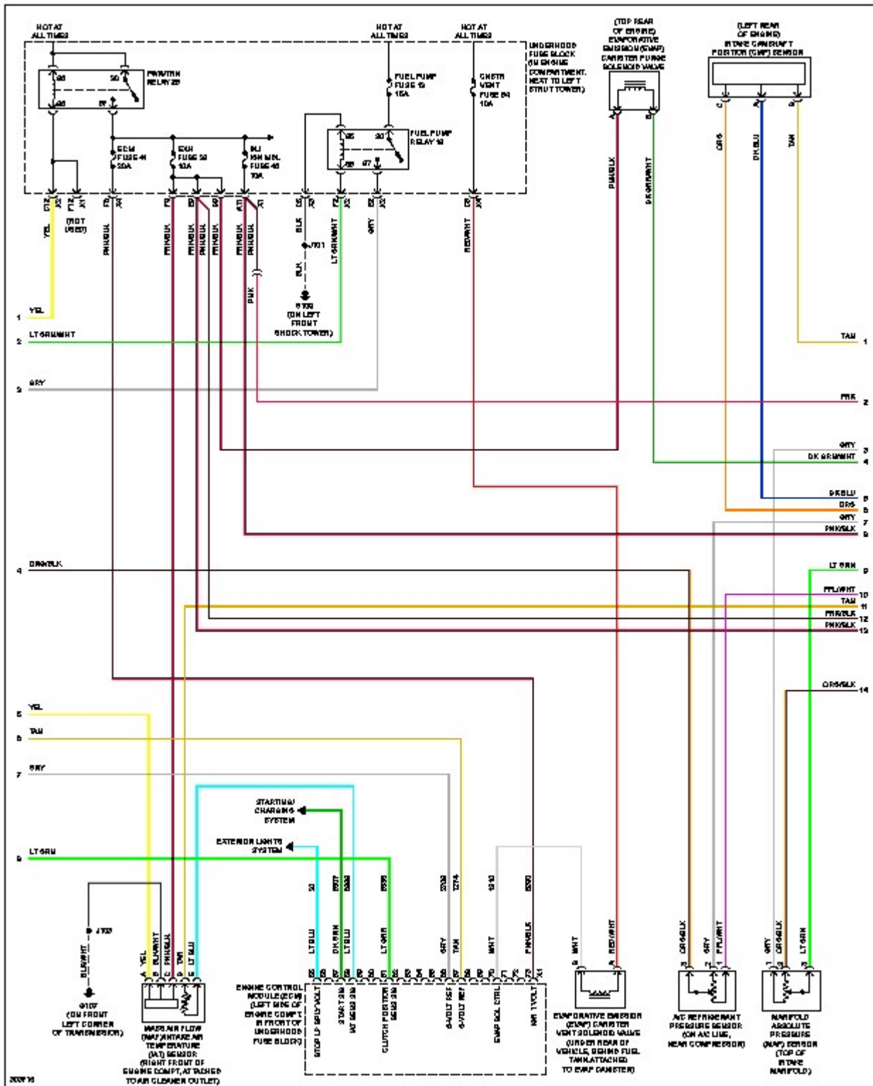
Fig. 26: 2.4L VIN V, Engine Performance Circuit (2 of 4)
