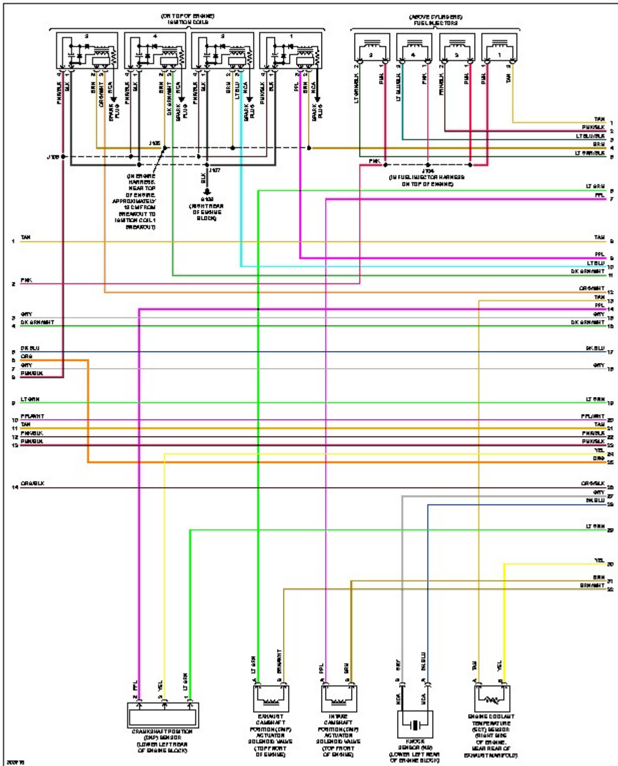
Fig. 27: 2.4L VIN V, Engine Performance Circuit (3 of 4)
