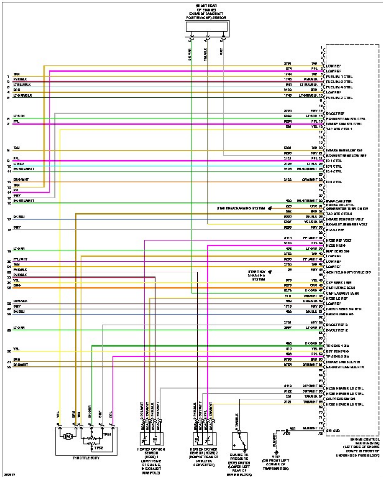
Fig. 28: 2.4L VIN V, Engine Performance Circuit (4 of 4)
