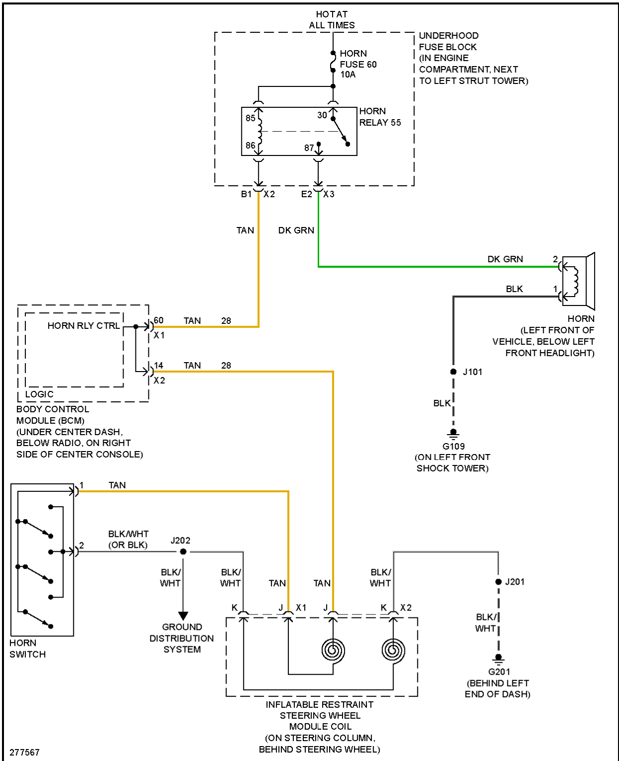
Fig. 33: Horn Circuit
