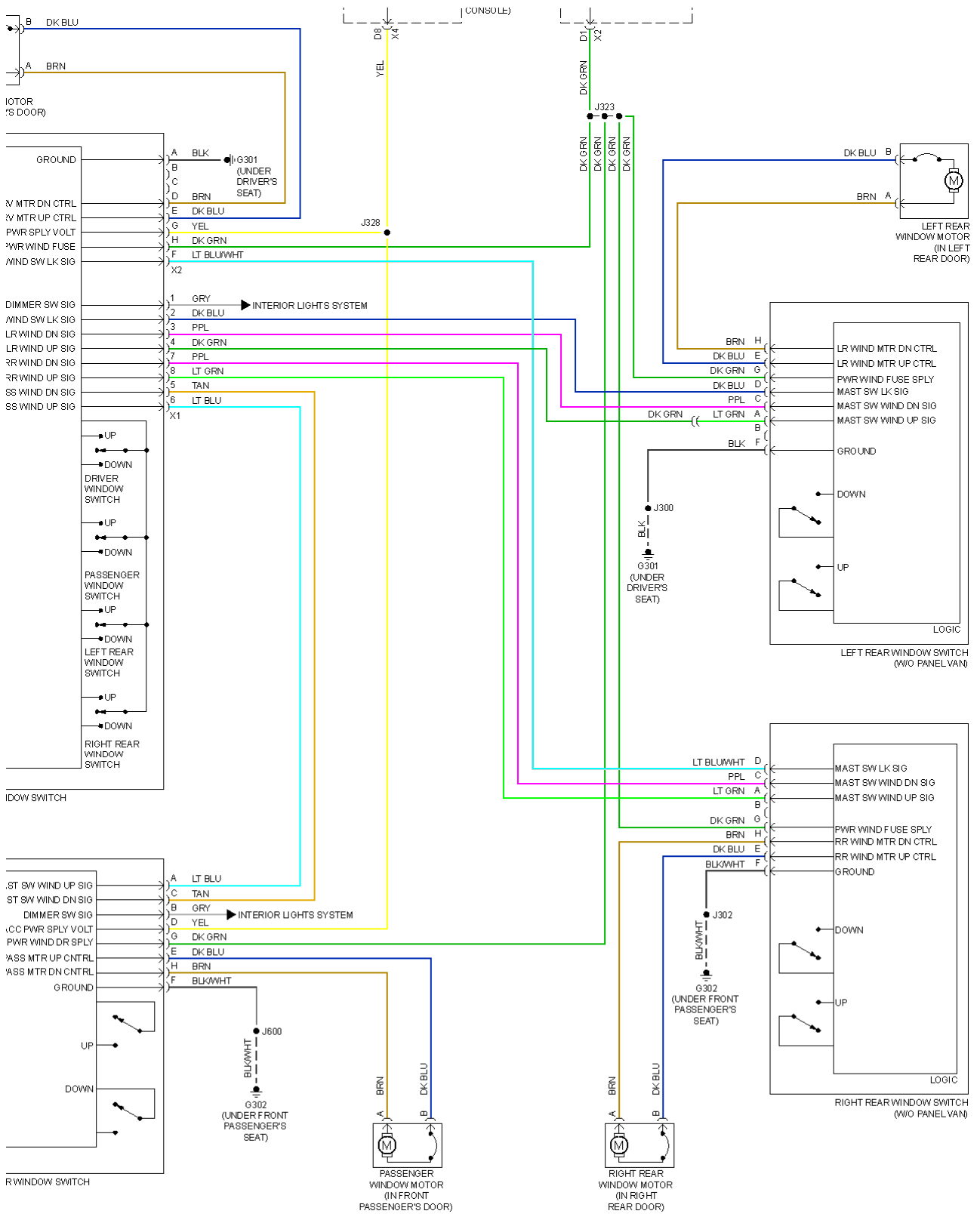
Fig. 53: Power Windows Circuit
