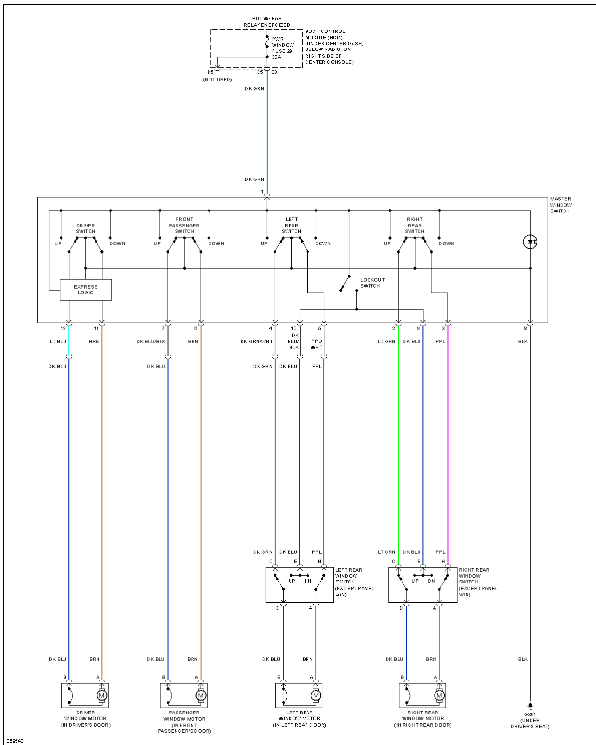
Fig. 43: Power Windows Circuit
